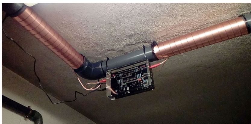
Vulcan S 10 - on the cold water main pipe
