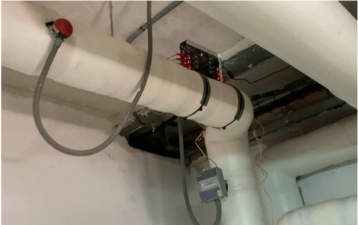
Vulcan S10 1 x water deposit line with Ø 63 mm
